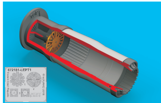
672 181 MiG-21MF exhaust nozzle
