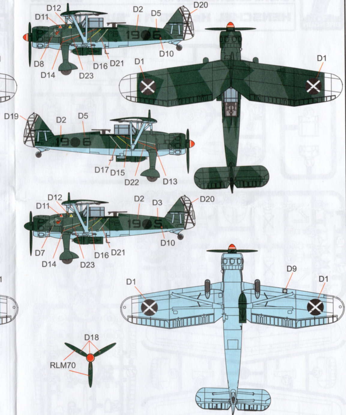
Hs 126A-1, 5.A/88 Legion Condor, Spain, 1938
