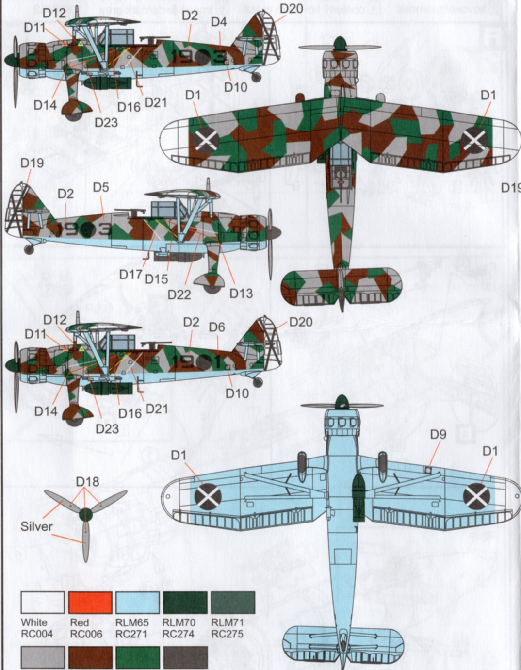
Hs 126A-1, 5.A/88 Legion Condor, Spain, 1938
