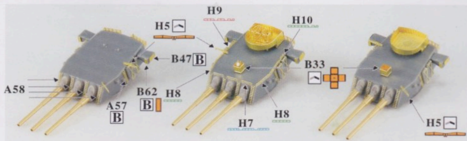
H7, H8, H9, 只安装在B炮塔 H7, H8, H9 only turret B
