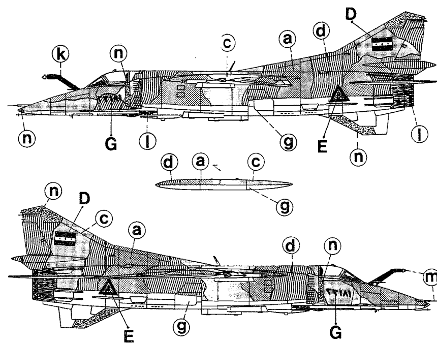
3 MiG-23BN Flogger H, Iraqi Air Force, Al Basrah West A.B., 1990-91, equipped with inflight-refueling probe and Exocet ASMs for anti-shiping operations.
