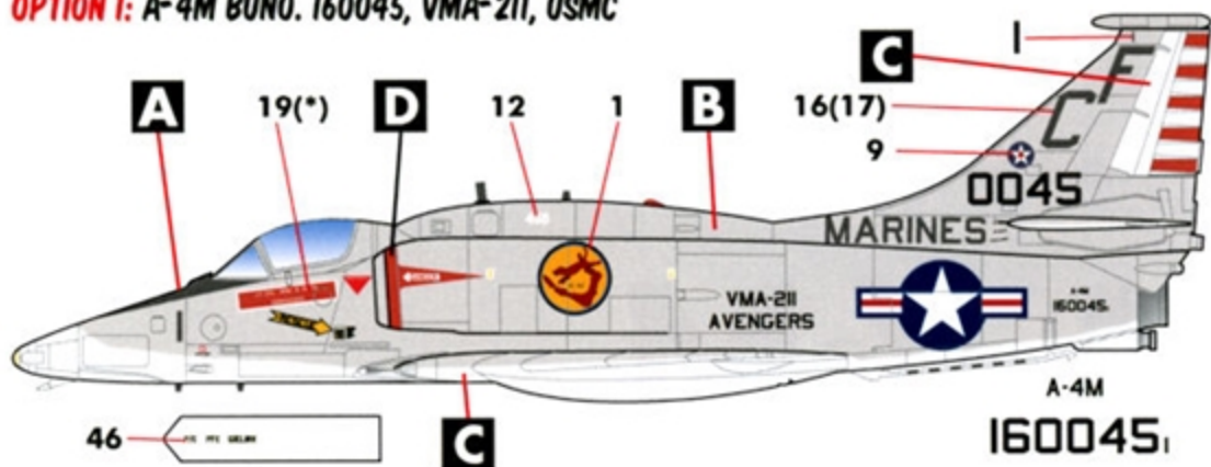
OPTION 1: A-4M BUNO. 160045, VMA-211, USMC
