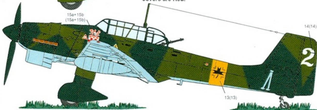
Ju 87B-2, 2nd Staffel, 1/StG 3, Greece, April 1941. Scheme is RLM 70/71 over RLM 65 with RLM 04 nose and rudder. Spinner is RLM 70 with Red tip and White stripe. Siren mount covers are Red.
